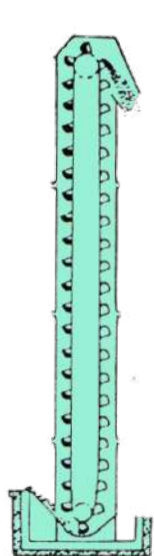
連續排出形 Continuous Bucket Elevator
